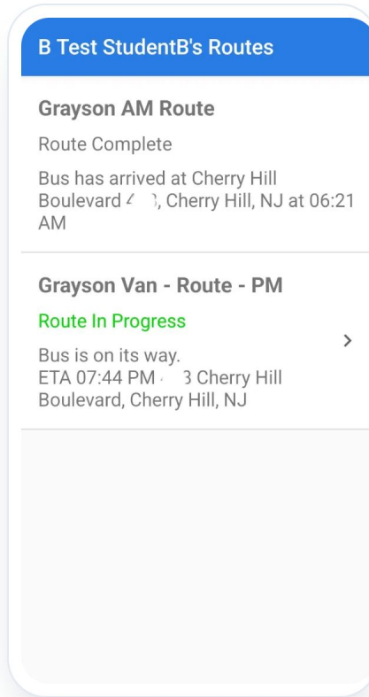
Boarding alerts
